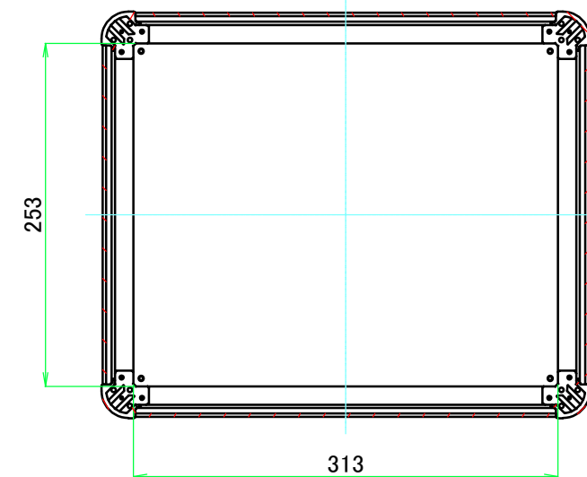
C-C (1:5)
