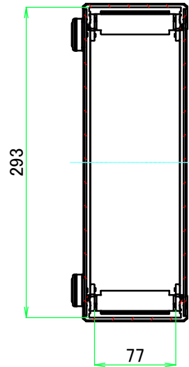
B-B (1:5)
